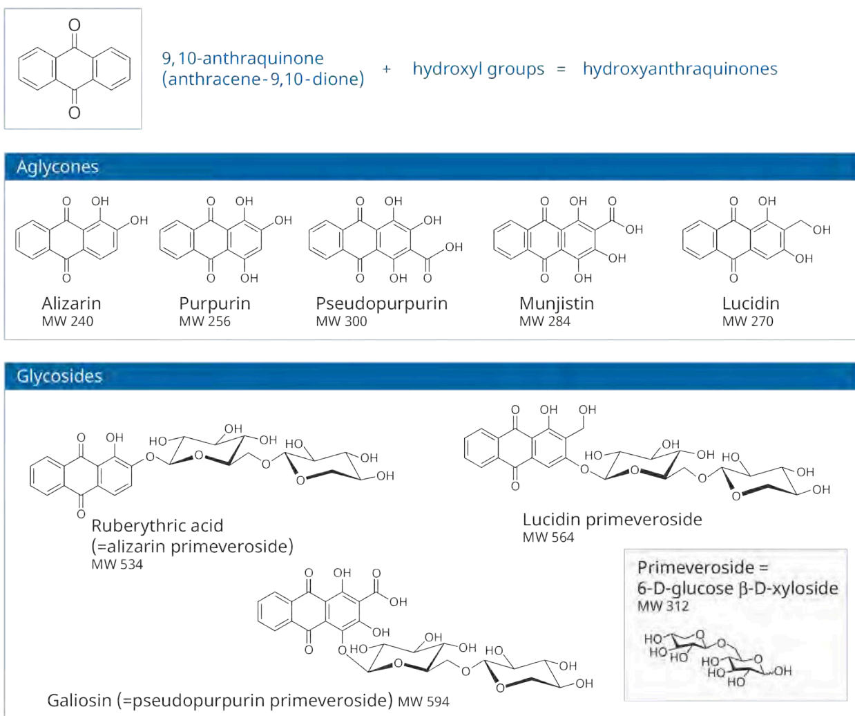
Figure 3.5 Structures (and molecular weights) of some common hydroxyanthraquinones and glycosides found in madder roots.
