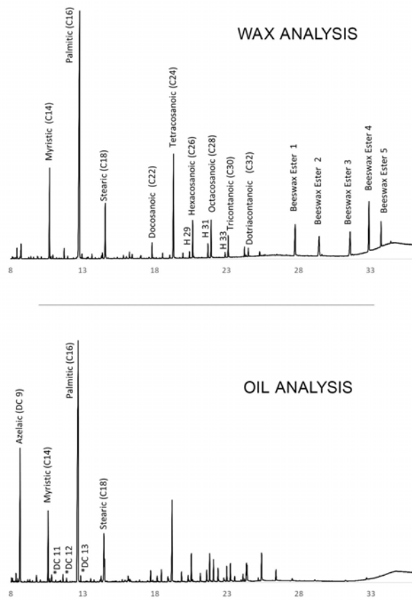
Figure 18.2b The GC/MS chromatograms for figure 18.2a show a sample containing aged beeswax, soaps, and oil. The top chromatogram presents the wax analysis; the bottom chromatogram displays the oil analysis of the same sample.
